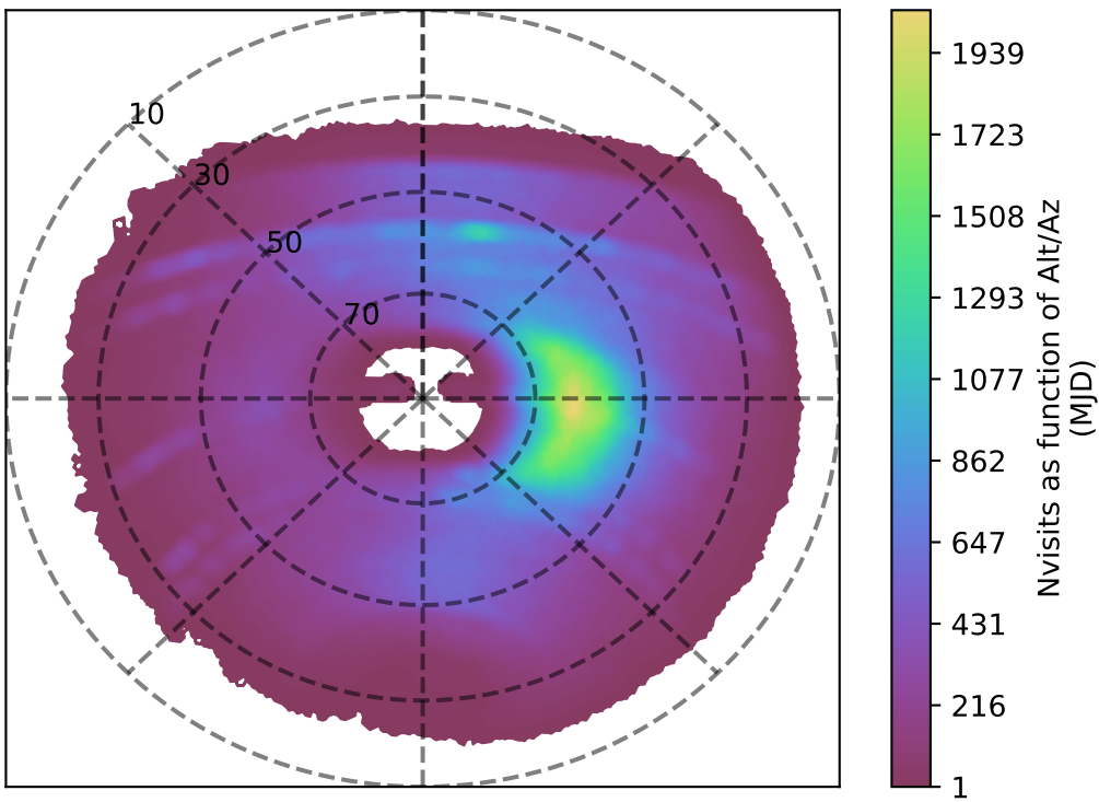
too_elab_r64_d3_griz_v3.4_10yrs y band: Nvisits as function of Alt/Az
