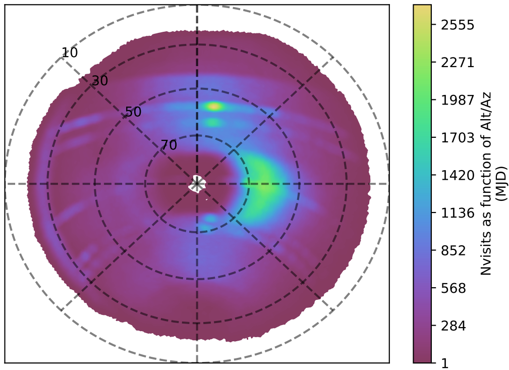
too_elab_r64_d3_griz_v3.4_10yrs r band: Nvisits as function of Alt/Az
