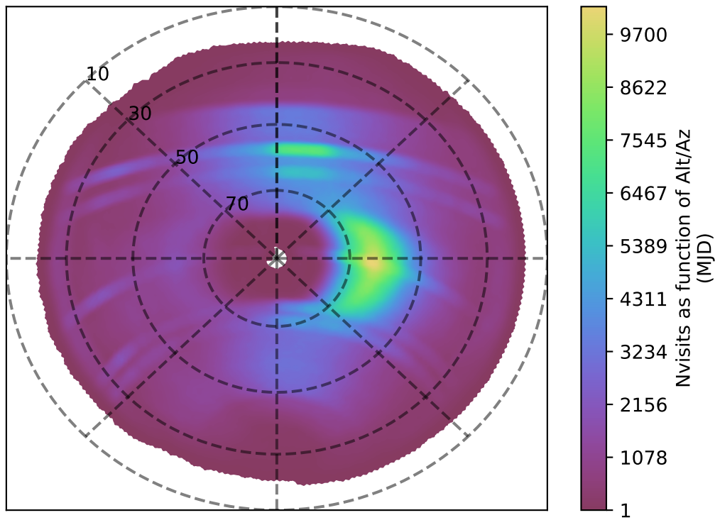
too_elab_r64_d3_griz_v3.4_10yrs all bands: Nvisits as function of Alt/Az
