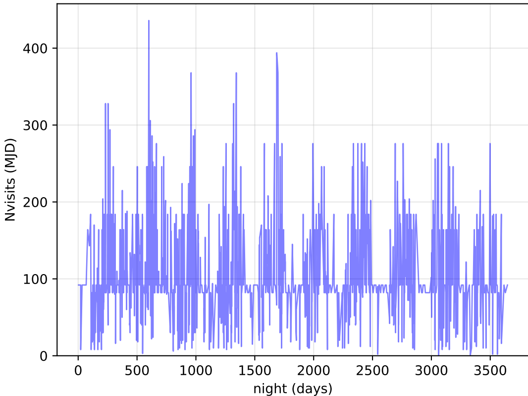
too_elab_r64_d3_griz_v3.4_10yrs DDF: Nvisits
