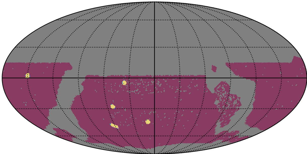
too_elab_r64_d3_griz_v3.4_10yrs WFD: NumberOfQuickRevisits
