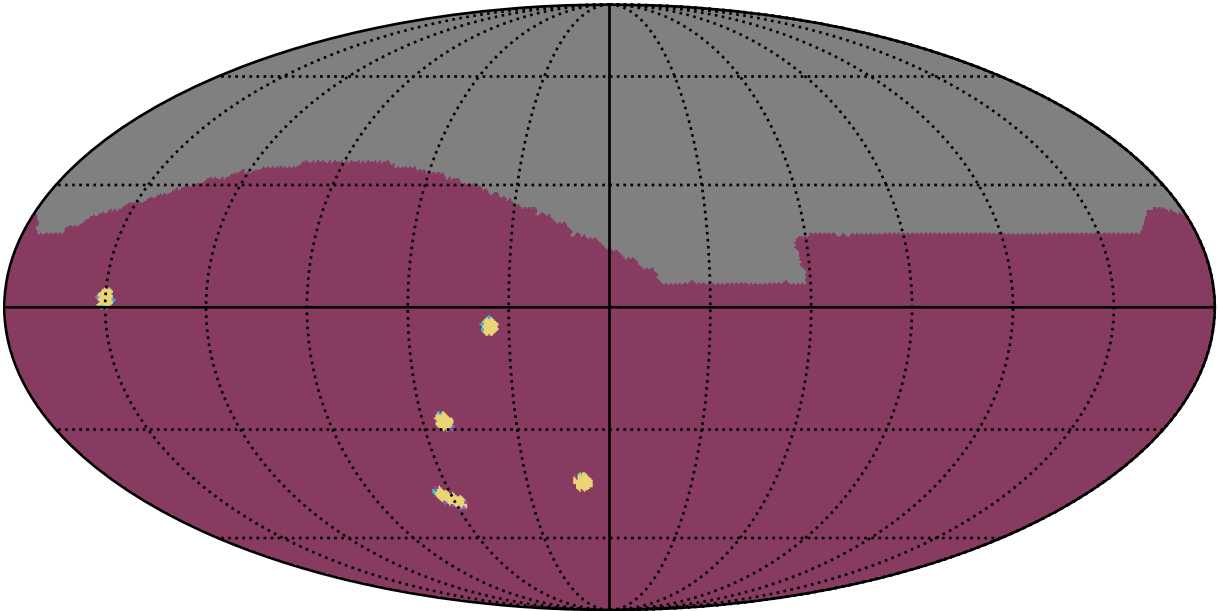
too_elab_r64_d3_griz_v3.4_10yrs All sky: NumberOfQuickRevisits
