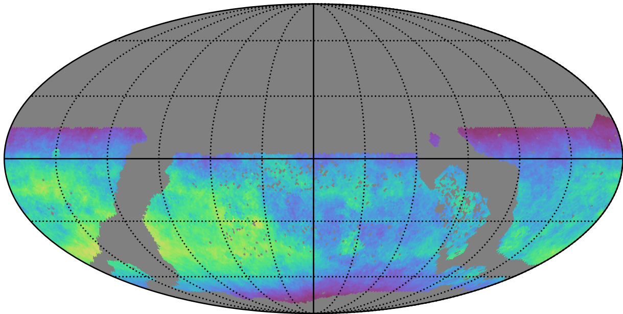
too_elab_r64_d3_griz_v3.4_10yrs WFD z band: Normalized Teff
