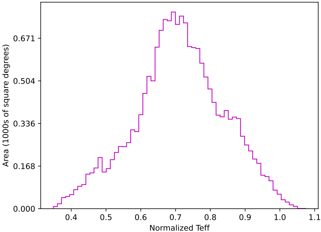
too_elab_r64_d3_griz_v3.4_10yrs WFD z band: Normalized Teff
