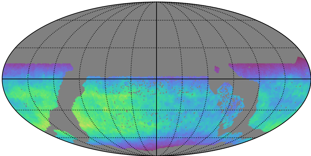
too_elab_r64_d3_griz_v3.4_10yrs WFD y band: Normalized Teff
