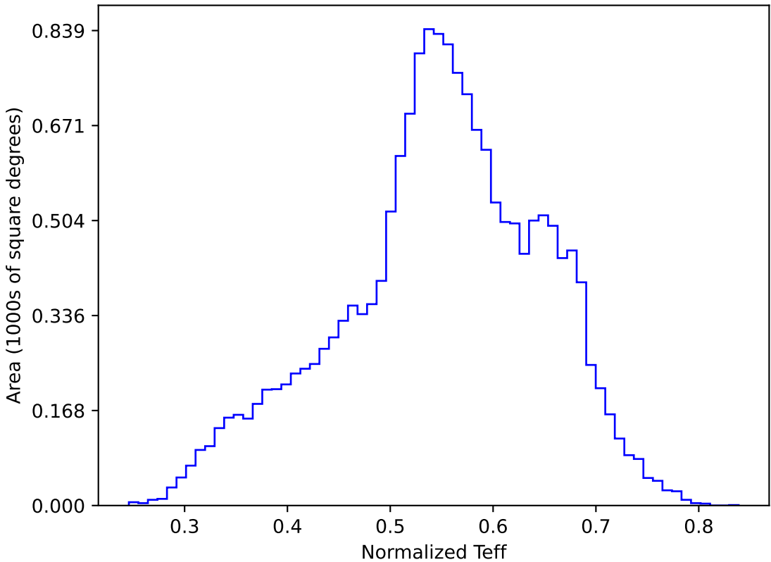
too_elab_r64_d3_griz_v3.4_10yrs WFD y band: Normalized Teff
