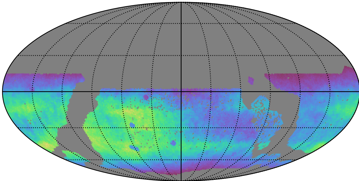
too_elab_r64_d3_griz_v3.4_10yrs WFD r band: Normalized Teff
