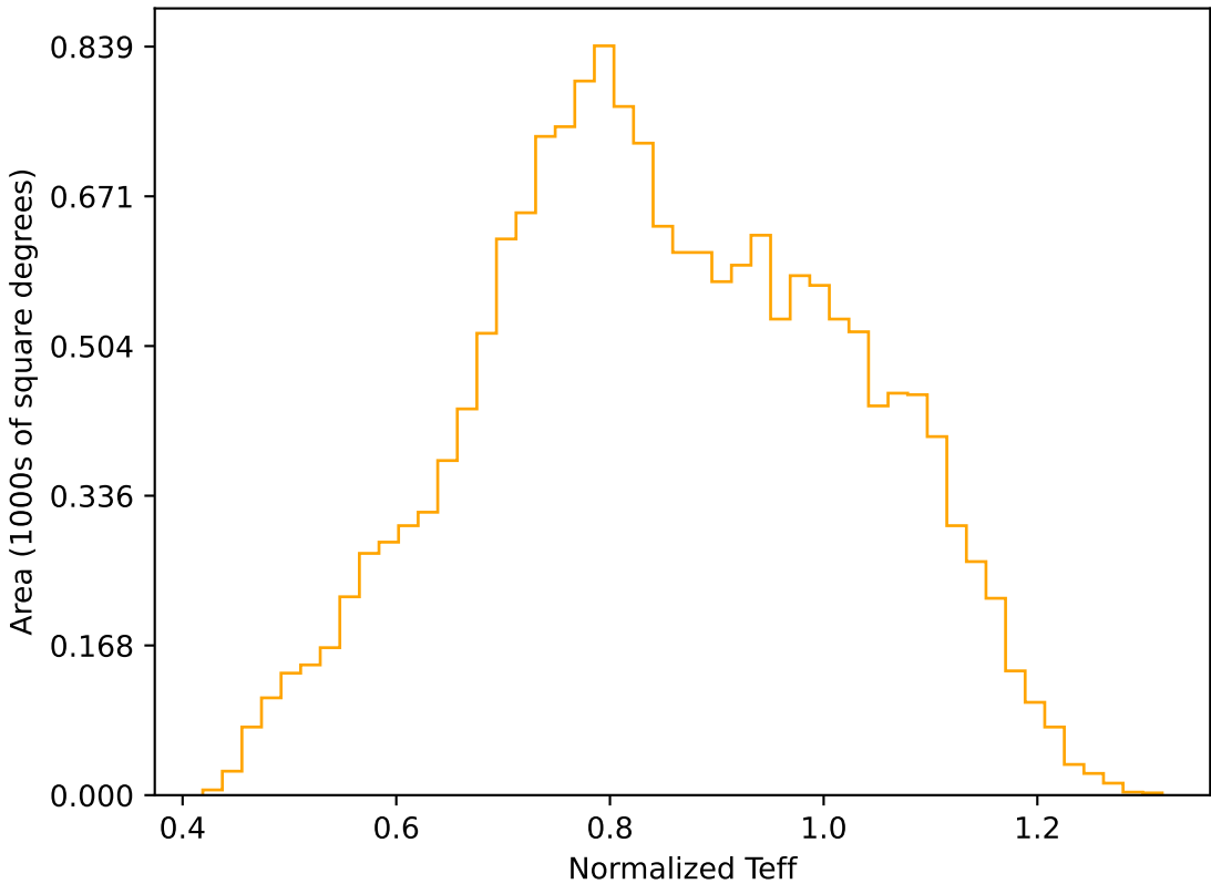
too_elab_r64_d3_griz_v3.4_10yrs WFD r band: Normalized Teff
