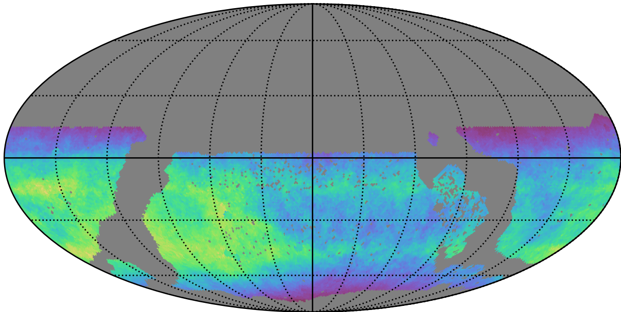
too_elab_r64_d3_griz_v3.4_10yrs WFD i band: Normalized Teff
