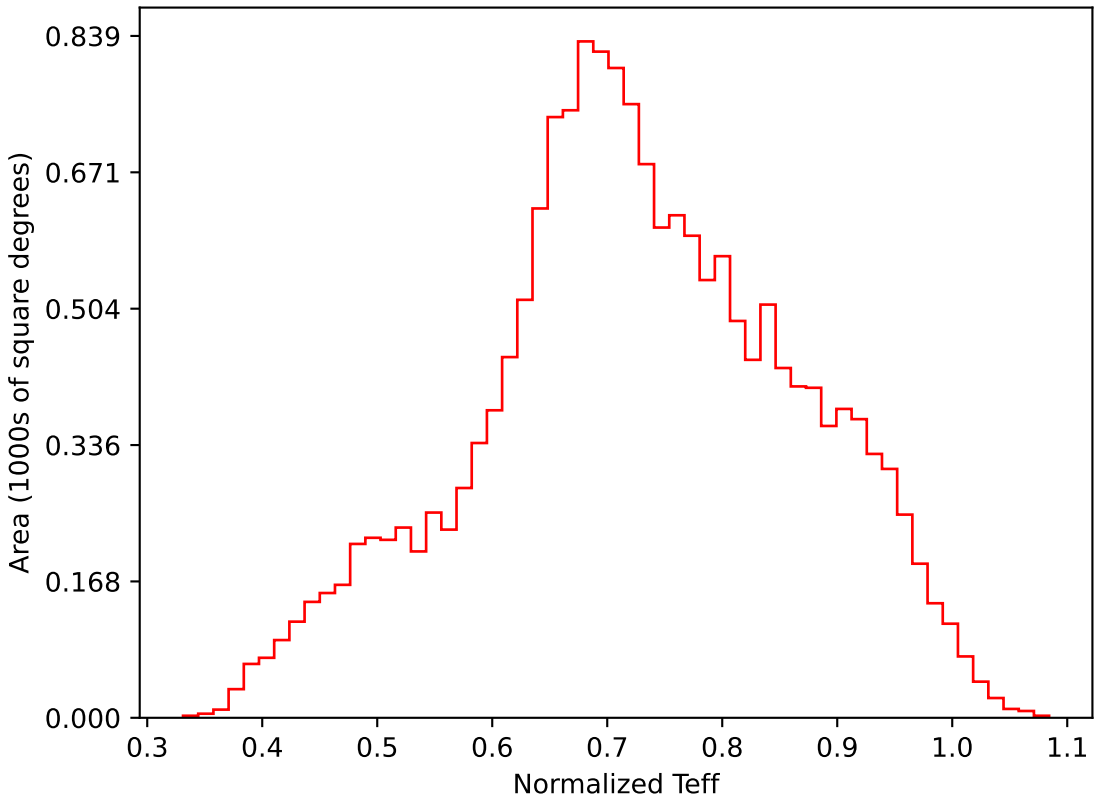
too_elab_r64_d3_griz_v3.4_10yrs WFD i band: Normalized Teff
