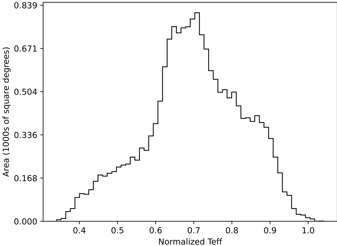
too_elab_r64_d3_griz_v3.4_10yrs WFD all bands: Normalized Teff
