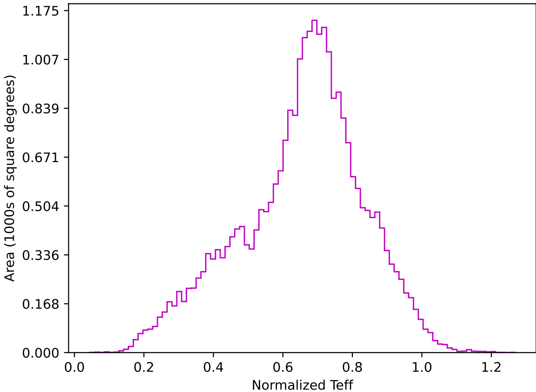
too_elab_r64_d3_griz_v3.4_10yrs All sky z band: Normalized Teff
