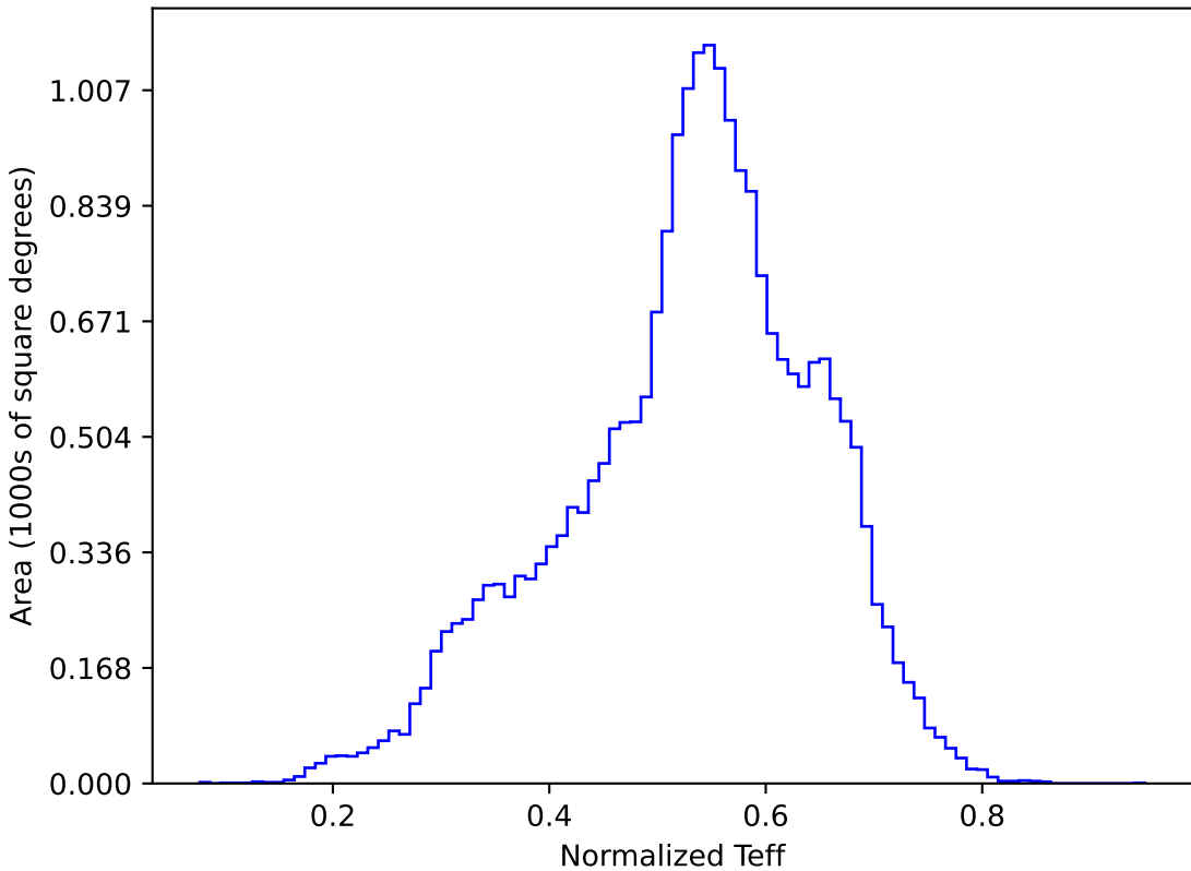
too_elab_r64_d3_griz_v3.4_10yrs All sky y band: Normalized Teff
