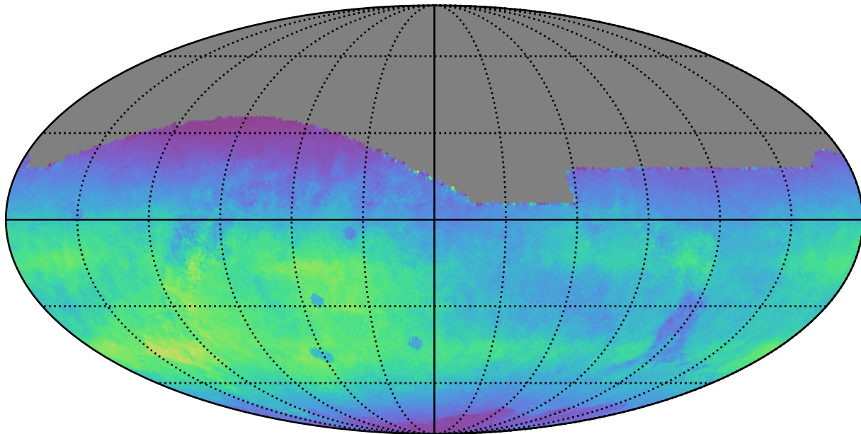
too_elab_r64_d3_griz_v3.4_10yrs All sky r band: Normalized Teff
