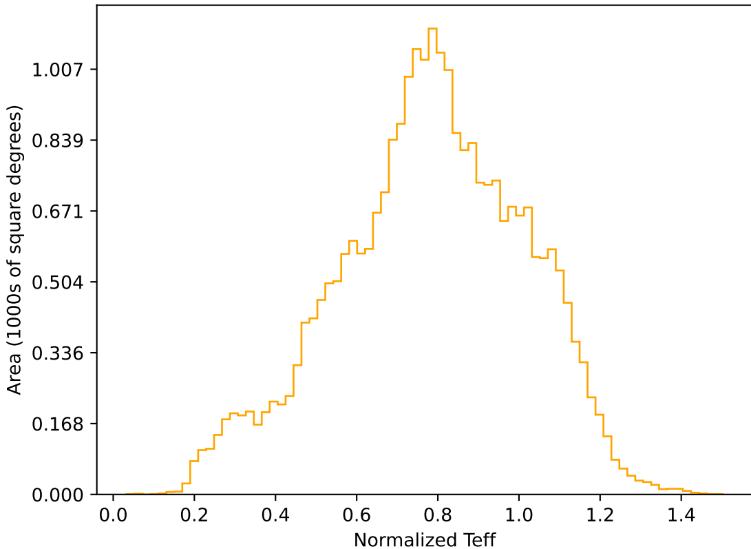
too_elab_r64_d3_griz_v3.4_10yrs All sky r band: Normalized Teff
