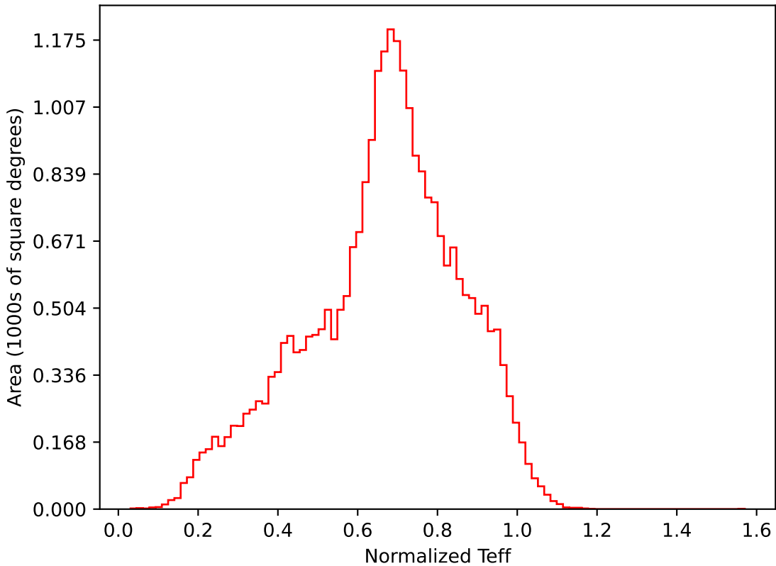
too_elab_r64_d3_griz_v3.4_10yrs All sky i band: Normalized Teff
