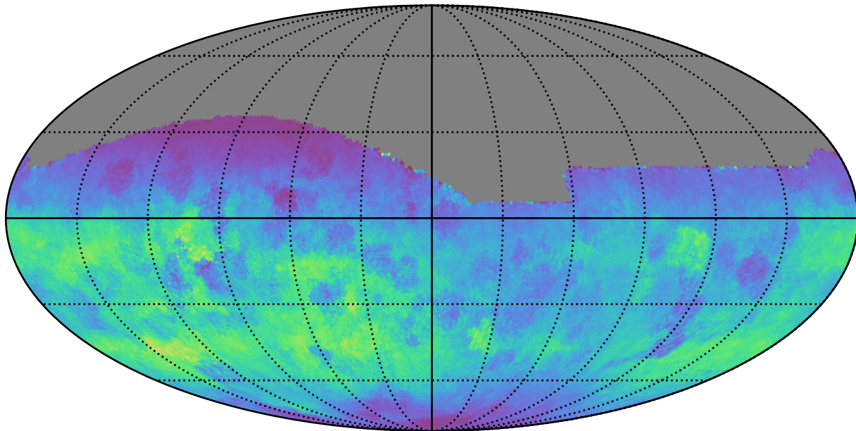
too_elab_r64_d3_griz_v3.4_10yrs All sky g band: Normalized Teff
