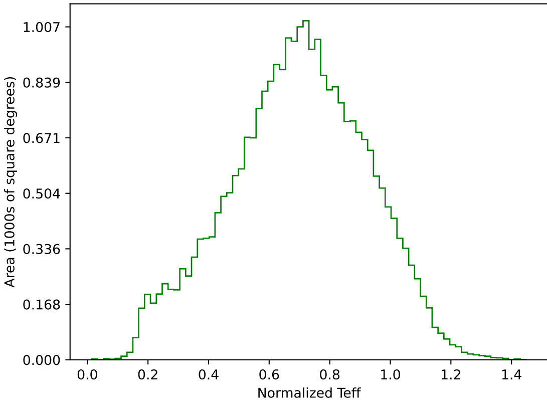
too_elab_r64_d3_griz_v3.4_10yrs All sky g band: Normalized Teff
