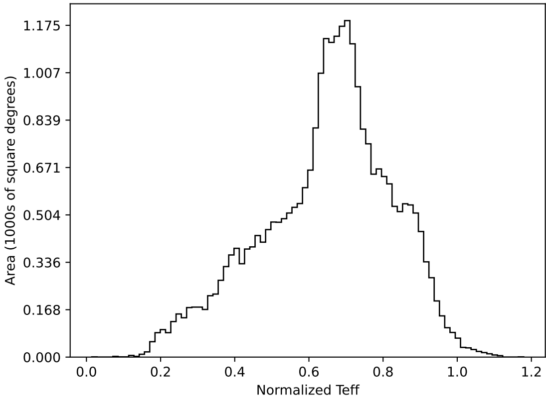
too_elab_r64_d3_griz_v3.4_10yrs All sky all bands: Normalized Teff
