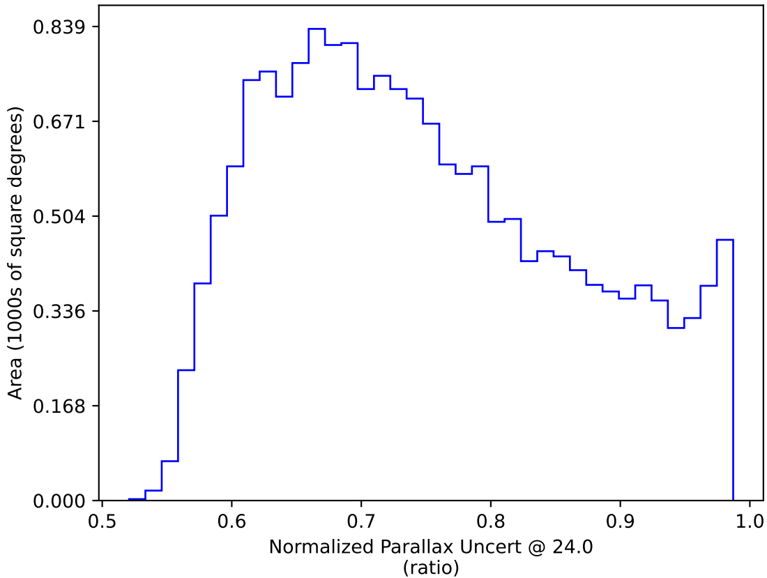
too_elab_r64_d3_griz_v3.4_10yrs WFD: Normalized Parallax Uncert @ 24.0
