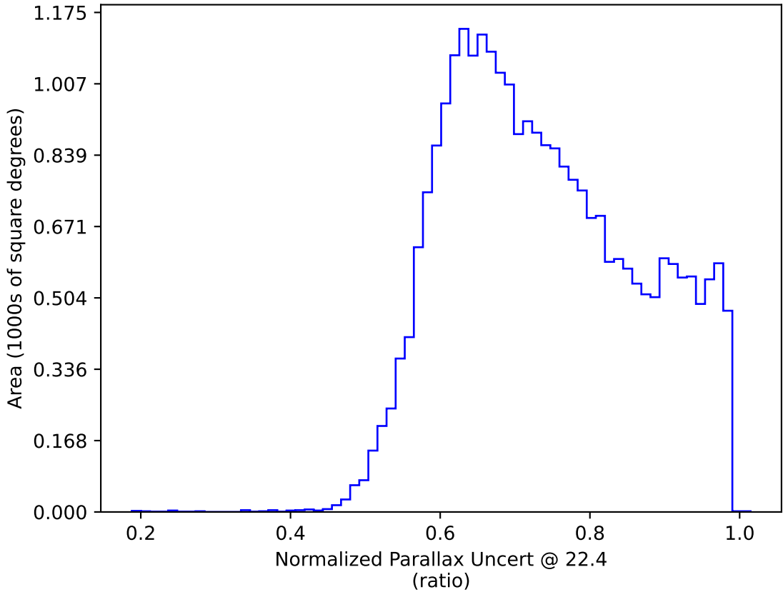
too_elab_r64_d3_griz_v3.4_10yrs All sky: Normalized Parallax Uncert @ 22.4
