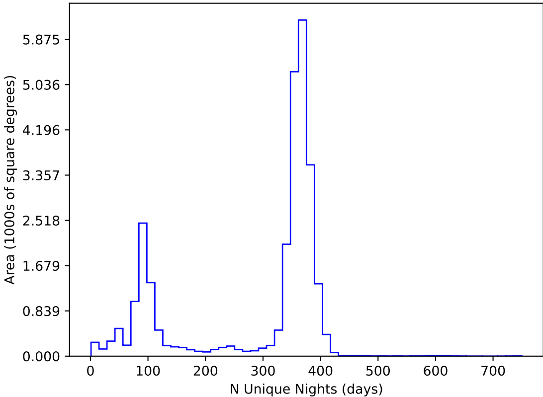
too_elab_r64_d3_griz_v3.4_10yrs All sky all bands: N Unique Nights
