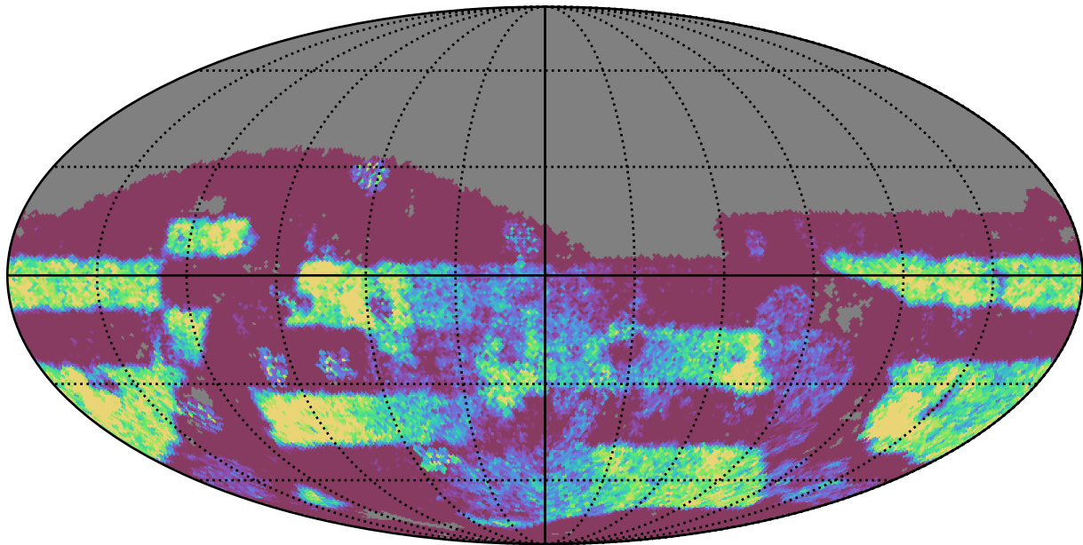
too_elab_r64_d3_griz_v3.4_10yrs Yr 3-4 z band: NVisits
