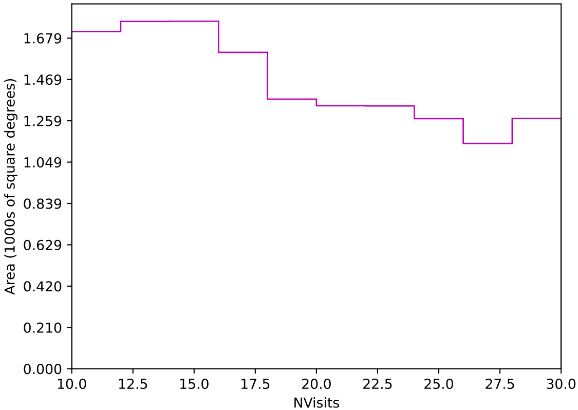
too_elab_r64_d3_griz_v3.4_10yrs Yr 3-4 z band: NVisits
