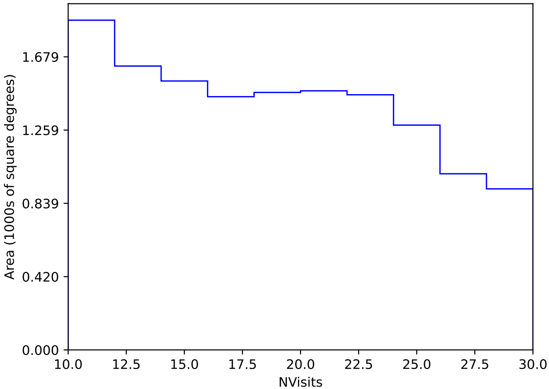
too_elab_r64_d3_griz_v3.4_10yrs Yr 3-4 y band: NVisits
