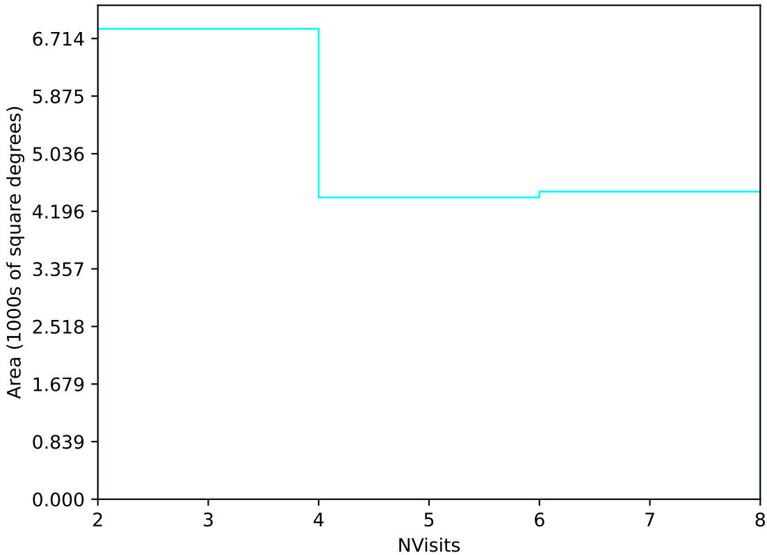
too_elab_r64_d3_griz_v3.4_10yrs Yr 3-4 u band: NVisits
