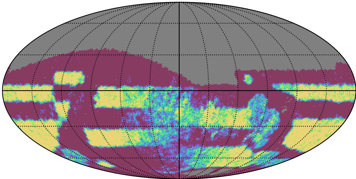
too_elab_r64_d3_griz_v3.4_10yrs Yr 3-4 r band: NVisits
