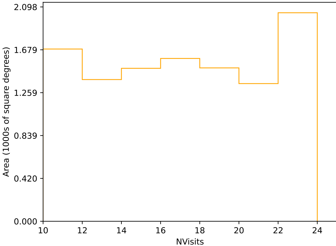
too_elab_r64_d3_griz_v3.4_10yrs Yr 3-4 r band: NVisits
