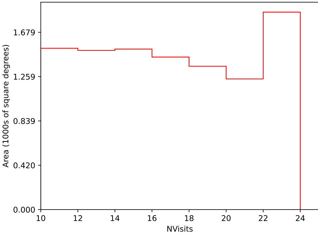
too_elab_r64_d3_griz_v3.4_10yrs Yr 3-4 i band: NVisits
