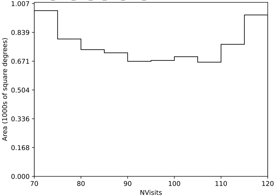
too_elab_r64_d3_griz_v3.4_10yrs Yr 3-4 all bands: NVisits
