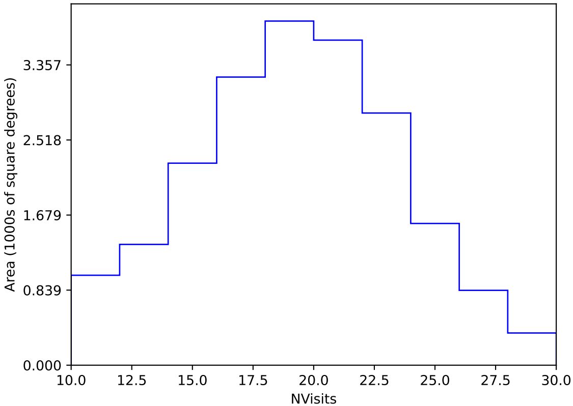
too_elab_r64_d3_griz_v3.4_10yrs Yr 1 y band: NVisits
