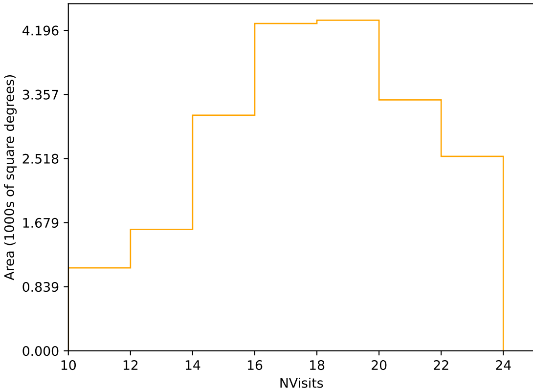
too_elab_r64_d3_griz_v3.4_10yrs Yr 1 r band: NVisits
