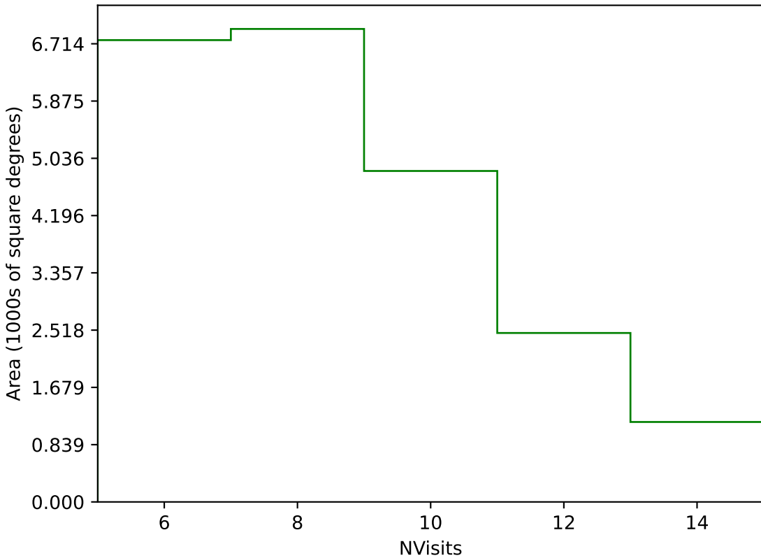
too_elab_r64_d3_griz_v3.4_10yrs Yr 1 g band: NVisits
