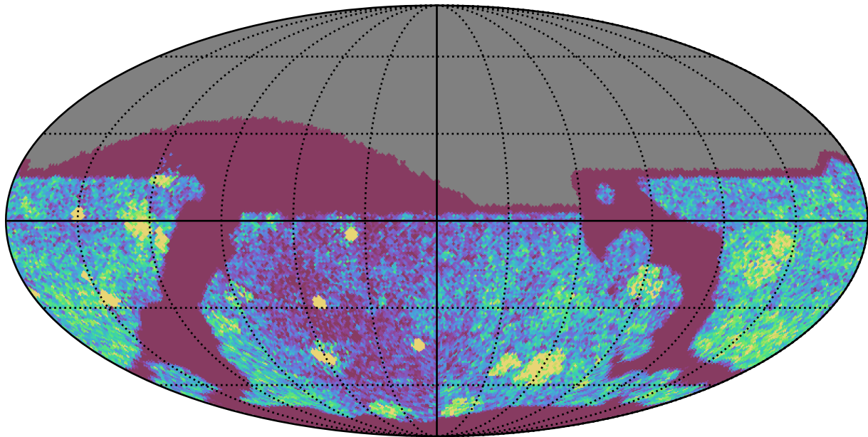
too_elab_r64_d3_griz_v3.4_10yrs Yr 1 all bands: NVisits
