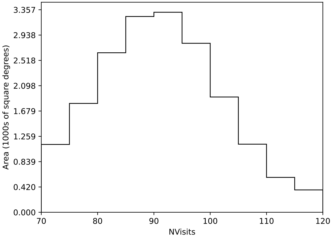
too_elab_r64_d3_griz_v3.4_10yrs Yr 1 all bands: NVisits
