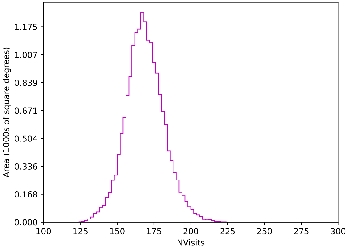
too_elab_r64_d3_griz_v3.4_10yrs WFD z band: NVisits
