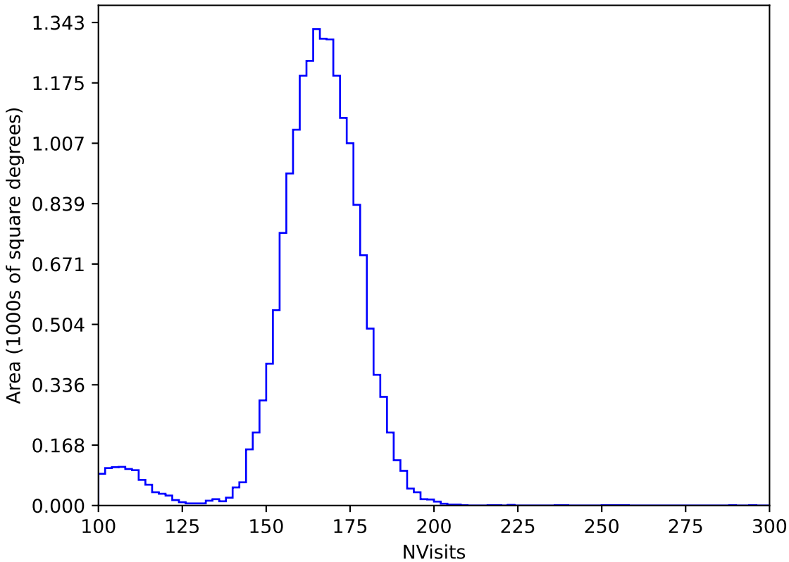
too_elab_r64_d3_griz_v3.4_10yrs WFD y band: NVisits
