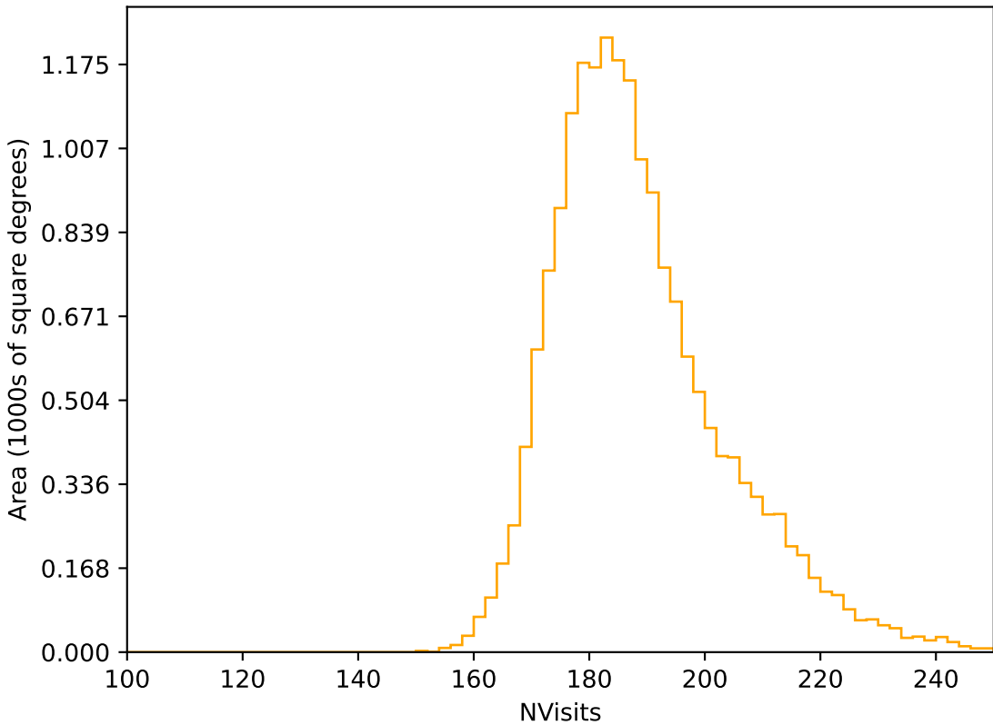
too_elab_r64_d3_griz_v3.4_10yrs WFD r band: NVisits
