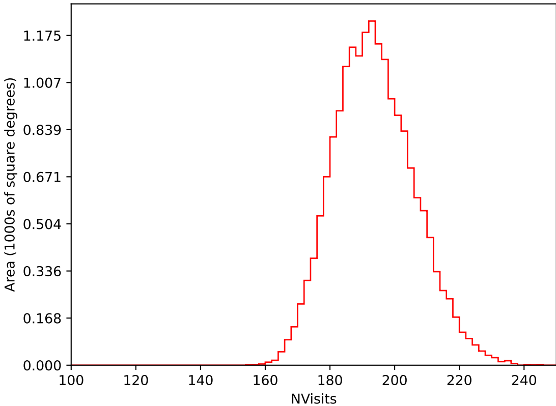
too_elab_r64_d3_griz_v3.4_10yrs WFD i band: NVisits
