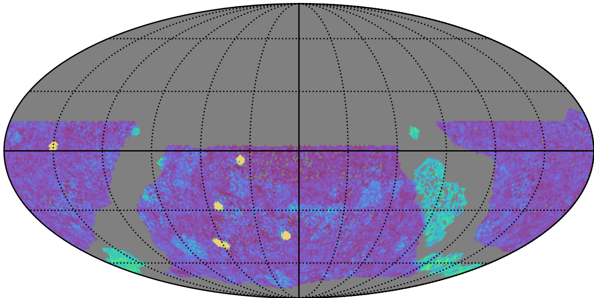
too_elab_r64_d3_griz_v3.4_10yrs WFD g band: NVisits
