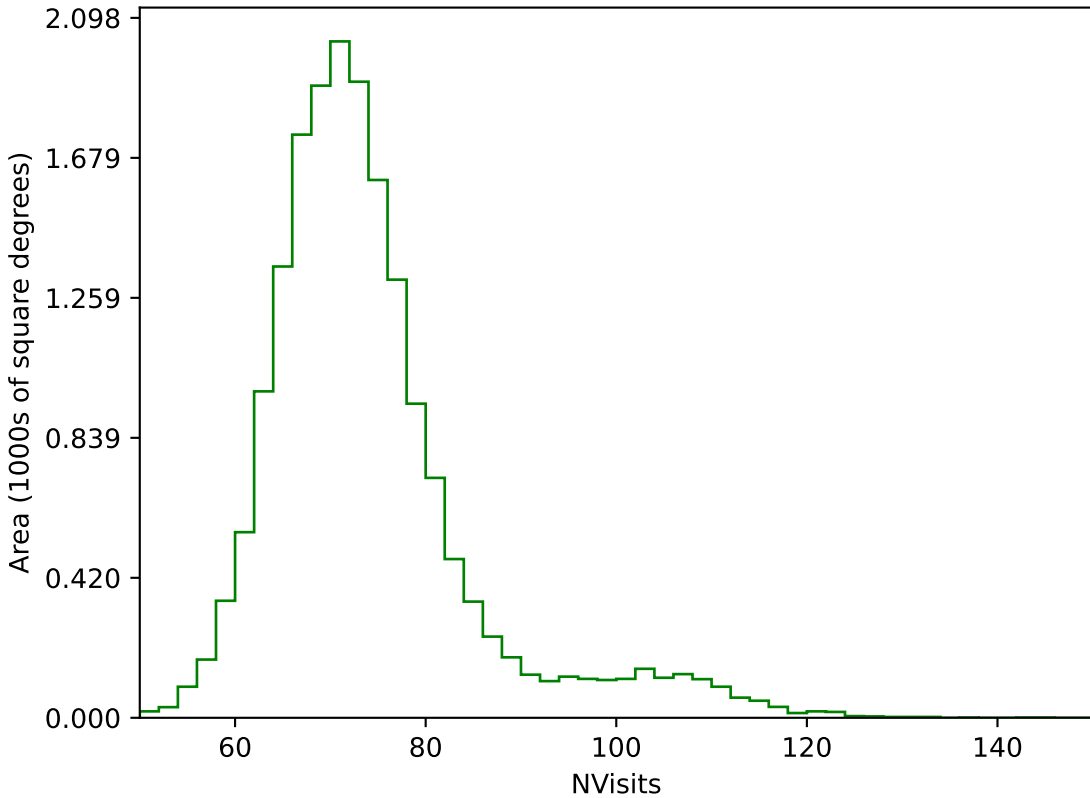
too_elab_r64_d3_griz_v3.4_10yrs WFD g band: NVisits
