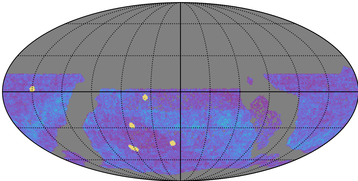
too_elab_r64_d3_griz_v3.4_10yrs WFD all bands: NVisits
