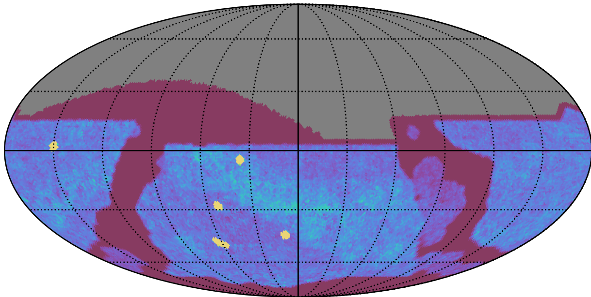
too_elab_r64_d3_griz_v3.4_10yrs All sky z band: NVisits
