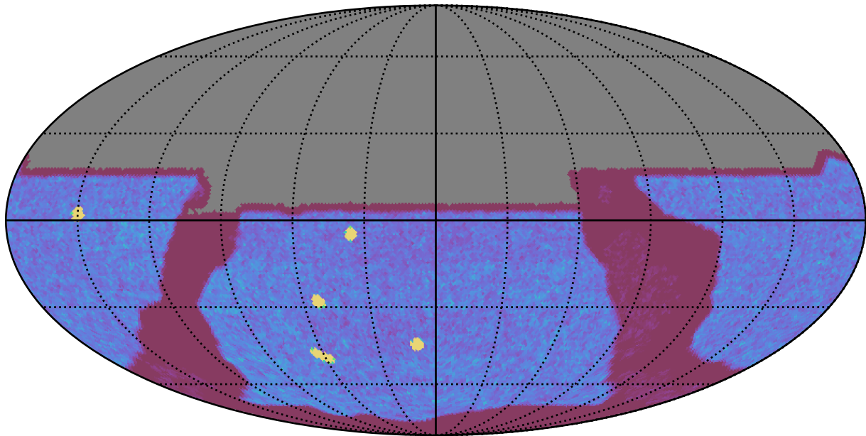
too_elab_r64_d3_griz_v3.4_10yrs All sky y band: NVisits
