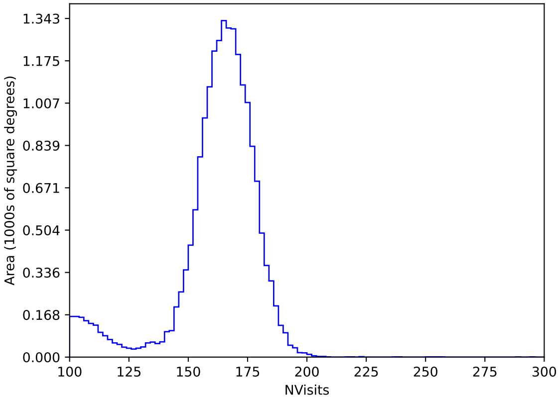
too_elab_r64_d3_griz_v3.4_10yrs All sky y band: NVisits
