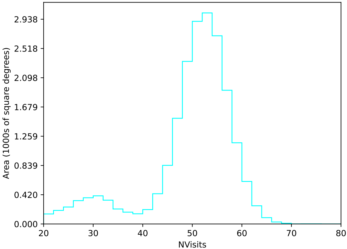
too_elab_r64_d3_griz_v3.4_10yrs All sky u band: NVisits
